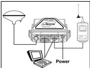
The drawing shows the GPS-Base connections.
