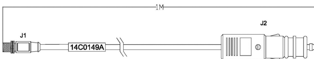
Figure 6. Cigar plug to M12 4 Pole Male pin 14C0149A
